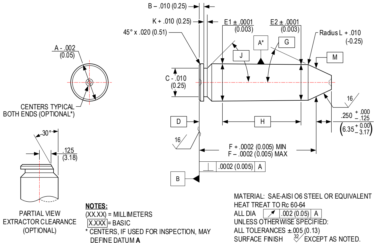
FIGURE I SHOULDER-BREECHING CENTERFIRE RIFLE HEADSPACE GAUGES
