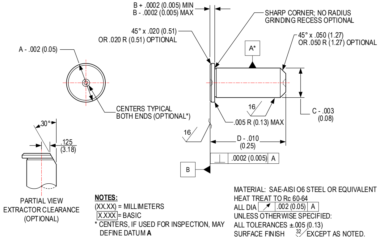
FIGURE III RIM-BREECHING CENTERFIRE RIFLE HEADSPACE GAUGES
