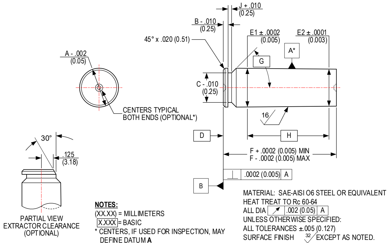
FIGURE IV MOUTH-BREECHING CENTERFIRE RIFLE HEADSPACE GAUGES
