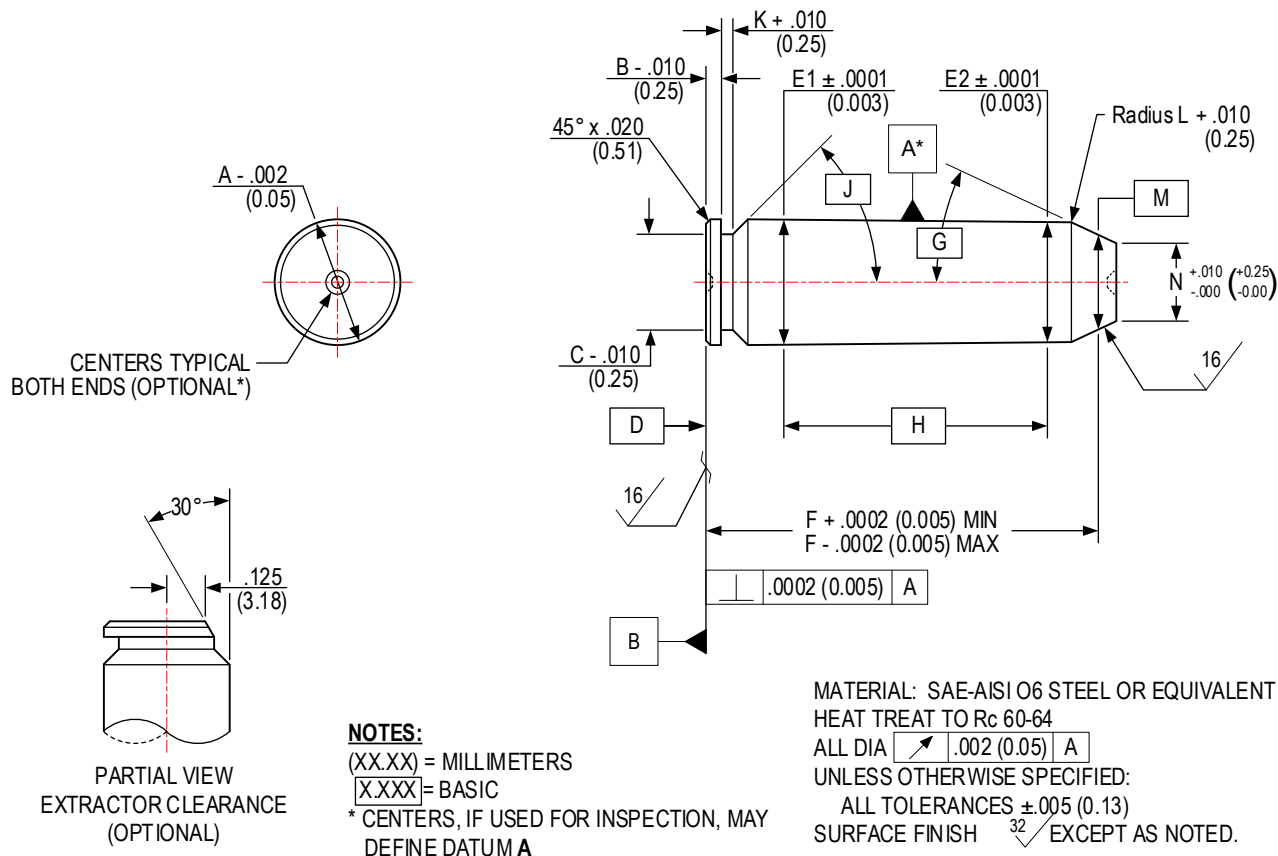
FIGURE V SHOULDER-BREECHING CENTERFIRE RIFLE HEADSPACE GAUGES (CARTRIDGE DESIGNS WITH NO INTEGRAL NECK)
